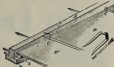
Van Reyper's Glazing Points
